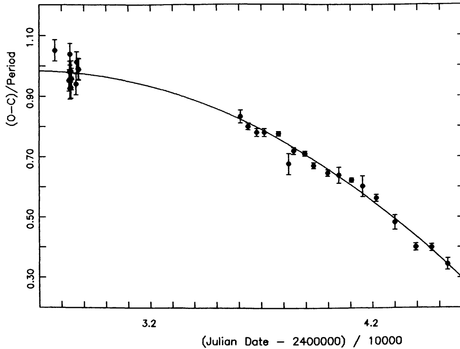
Figure 2. O-C graph for V1303 Sgr with least squares parabola, using all of the available data. The data within the range JD 2427000-2429000 are by Oosteroff and Horikx (1954). The point at JD 2438230 is from Kwee and Braun. The rest are from Maria Mitchell Observatory plates.
