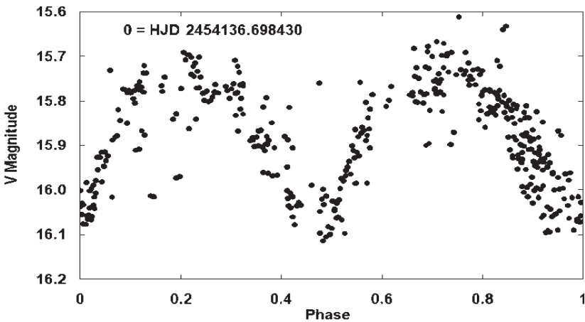
Figure 6. Phased differential photometry for USNO-B1.0 1057-0097388. Period = 9.3576 hours.
